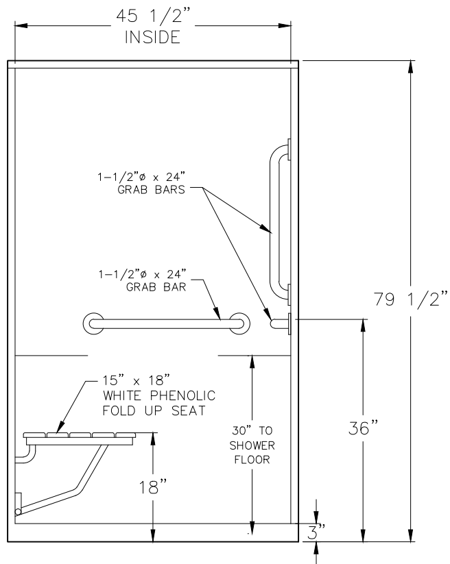
FRONT
