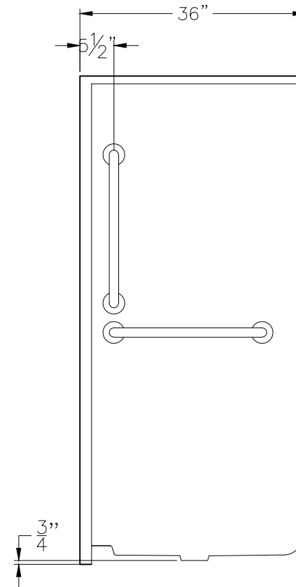
SIDE
